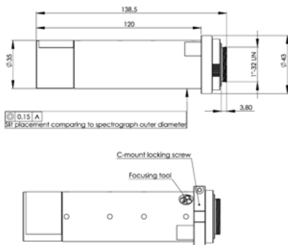
ImSpector V8/V10 mechanical dimensions
